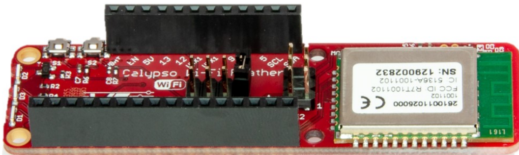
Figure 1: The WE Calypso FeatherWing (2610039025001)
