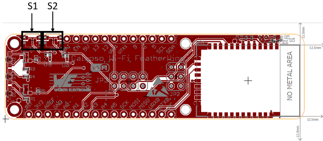
Figure 4: Push buttons
