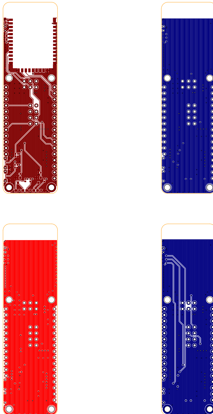
Figure 7: Top, bottom and internal layers
